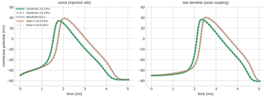
Figure 6: Do the three simulators integrate the same model? One cell’s first action potential, at the soma and at the far end of the dendrite, which moves only if axial coupling is integrated. Each simulator is drawn twice, one backend wide and pale with the other dashed on top, so a coinciding pair reads as agreement rather than a missing line. NEURON and Arbor agree to 0.02 mV at the peak and 0.01% on rate; GENESIS peaks 4.6 mV lower, its Hodgkin–Huxley rates being written about a -70 mV rest where NEURON’s use -65 . Data: cluster_bringup/logs/vmcross/ .
