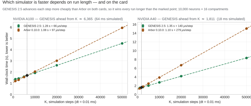
Figure 5: Both simulators are linear in K , so they cross, and a comparison at a single run length reports whichever side of the crossing the author happened to choose. The crossing sits earlier on the A40 because our kernel is fp32 where Arbor computes in double, and that card’s double-precision throughput is a fraction of the A100’s. N = 10\,000 neurons \times 16 compartments, mean \pm std over 3 replicates.
