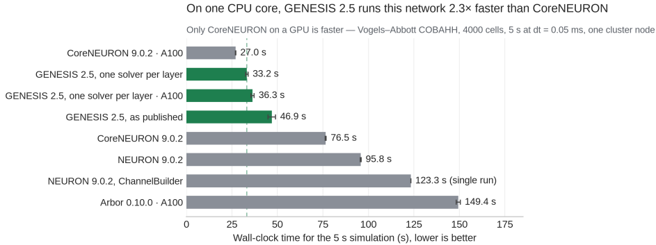
Figure 4: The measurements of Table 5, drawn. Green is GENESIS, grey the simulators it is compared against; each label names the device, and the dashed guide marks the fastest GENESIS time, so every bar reaching past it is slower. Means of 3 replicates with standard deviations, except the ChannelBuilder row. Arbor comes last despite its GPU because zero axonal delay forces it to exchange spikes every step.
