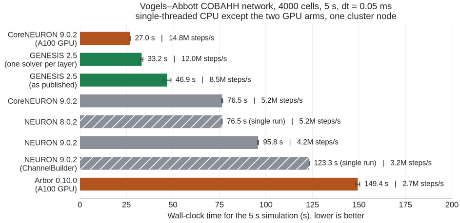
Figure 4: GENESIS 2.5 against NEURON, CoreNEURON and Arbor on the Vogels–Abbott COBAHH network, one UMCS node. All arms are single-threaded CPU except the two coloured apart, CoreNEURON and Arbor on an A100. Hatched bars are single runs; the others are means of 3 replicates with standard deviations. Throughput is quoted over the 4 \times 10^8 neuron-steps the 5 s simulation advances. Against CoreNEURON on CPU the GENESIS arm completes the network in two thirds of the time using no accelerator at all, and in under half once built as one solver per layer; against CoreNEURON on the GPU it remains behind.
