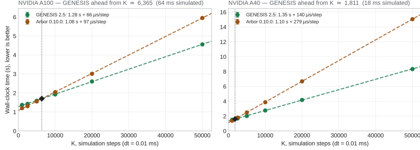
Figure 5: Neither simulator is faster in general: which one wins depends on how long the run is, and where the changeover falls depends on the card. Both are linear in K — Arbor starts about 0.2s ahead on setup, GENESIS 2.5 advances each step more cheaply — so a comparison at a single run length reports whichever side of the crossing the author happened to choose. Our per-step margin is the wider one on the A40, 140 against Arbor’s 279 \mu s, where on the A100 it is 66 against 97; the crossing moves accordingly, from K \approx 6400 to K \approx 1800 . Our kernel is fp32 where Arbor computes in double, and the A40’s double-precision throughput is a fraction of the A100’s. N = 10\,000 neurons \times 16 compartments, mean \pm std over 3 replicates.
