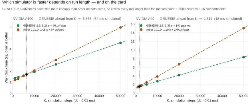
Figure 5: Wall-clock time against run length for the multi-compartment benchmark, one panel per card, N = 10\,000 neurons \times 16 compartments, mean \pm std over 3 replicates. The dotted line and diamond mark where the fitted lines cross.
