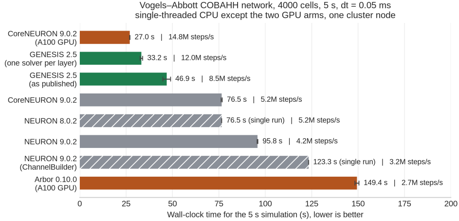
Figure 4: Where GENESIS 2.5 sits among the other simulators on the Vogels–Abbott COBAHH network, one UMCS node. Every arm is single-threaded CPU except the two coloured apart, CoreNEURON and Arbor on an A100; hatched bars are single runs, the rest means of 3 replicates. On the same core GENESIS is the fastest of the four — two thirds of CoreNEURON’s time as published, under half once built as one solver per layer — but CoreNEURON on the GPU stays ahead of all of them.
