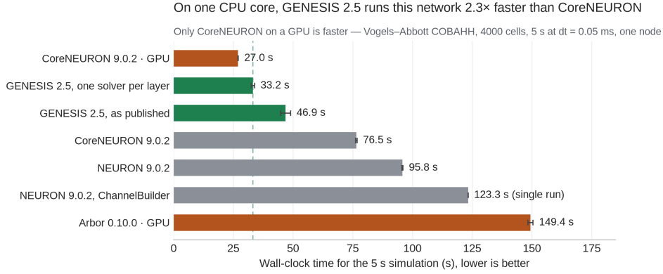
Figure 4: The measurements of Table 5, drawn. Green is GENESIS, orange the arms running on an A100, grey the CPU arms it is compared against; the dashed guide marks the GENESIS time, so every bar reaching past it is slower. Means of 3 replicates with standard deviations, except the ChannelBuilder row. Arbor comes last despite its GPU because zero axonal delay forces it to exchange spikes every step.
