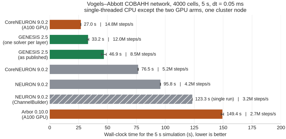
Figure 4: Where GENESIS 2.5 sits among the other simulators on the Vogels–Abbott COBAHH network, one UMCS node. Every arm is single-threaded CPU except the two coloured apart, CoreNEURON and Arbor on an A100; the hatched bar is a single run, the rest means of 3 replicates. On the same core GENESIS is the fastest of the four — two thirds of CoreNEURON’s time as published, under half once built as one solver per layer — but CoreNEURON on the GPU stays ahead of all of them.
