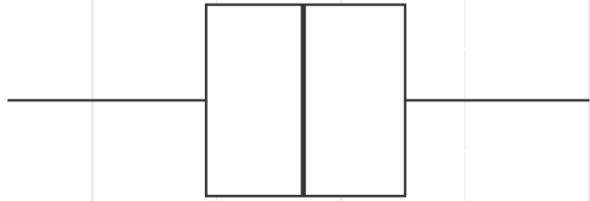
2 Permutations
