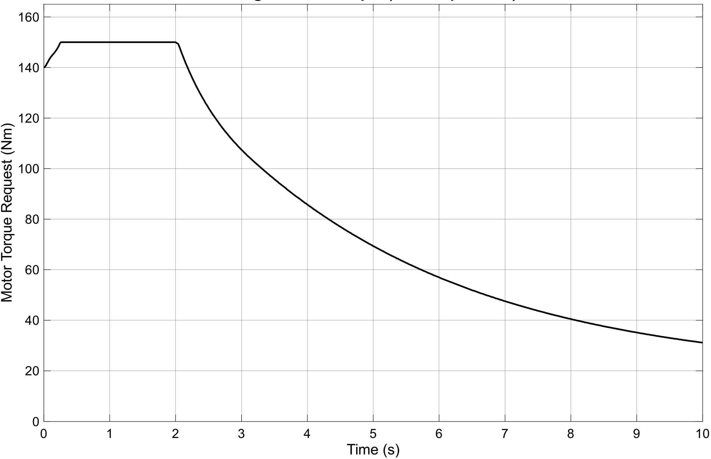
Target Motor Torque (1.00 Grip Factor)
