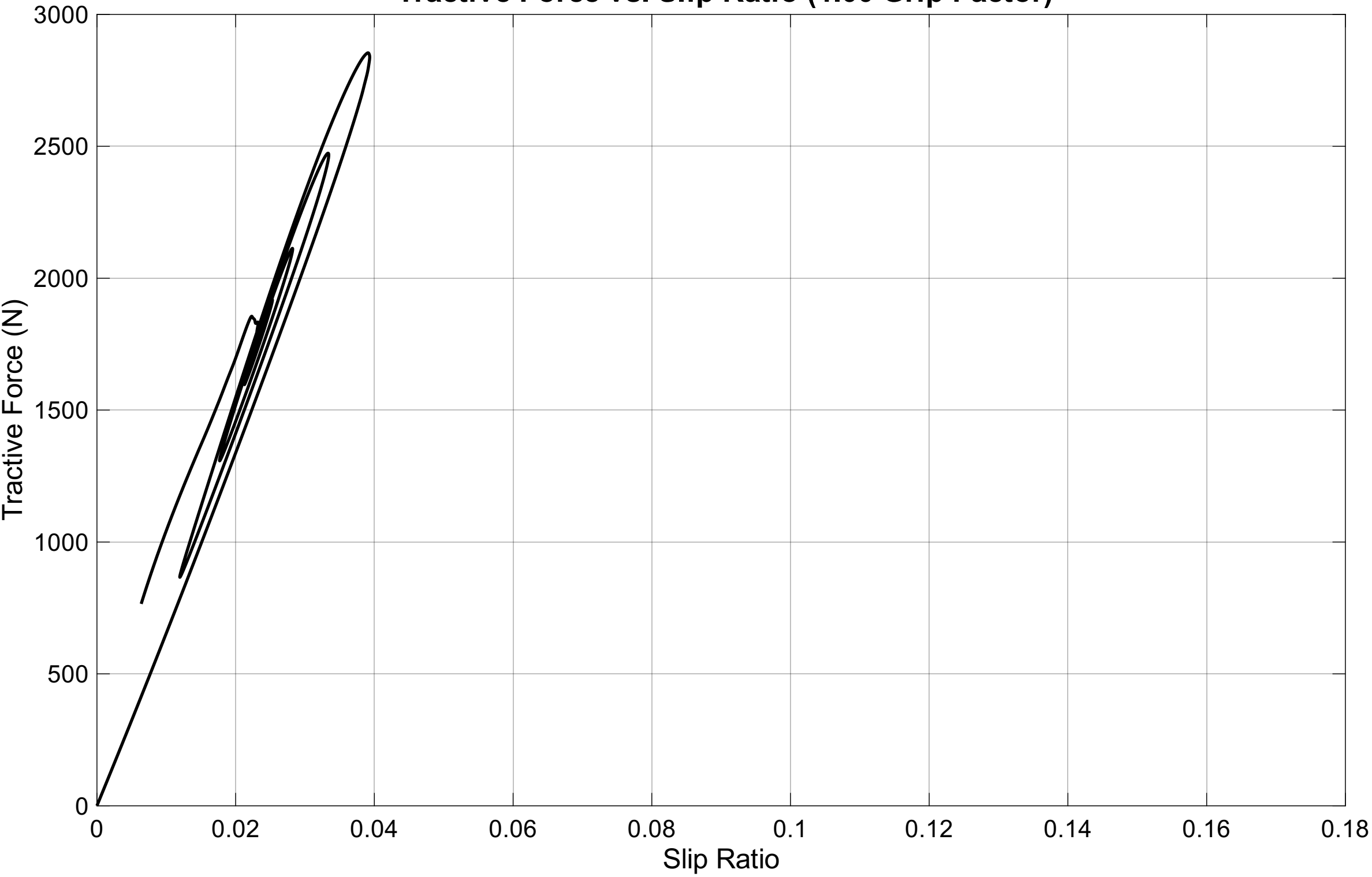
Tractive Force vs. Slip Ratio (1.00 Grip Factor)
