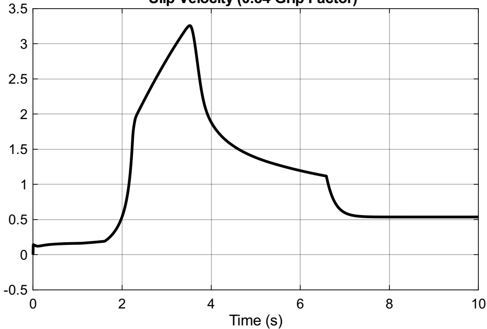
Slip Velocity (0.84 Grip Factor)
