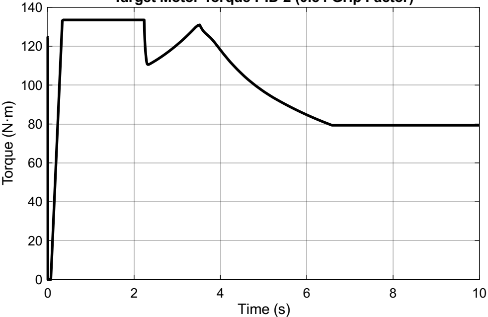
Target Motor Torque PID 2 (0.84 Grip Factor)
