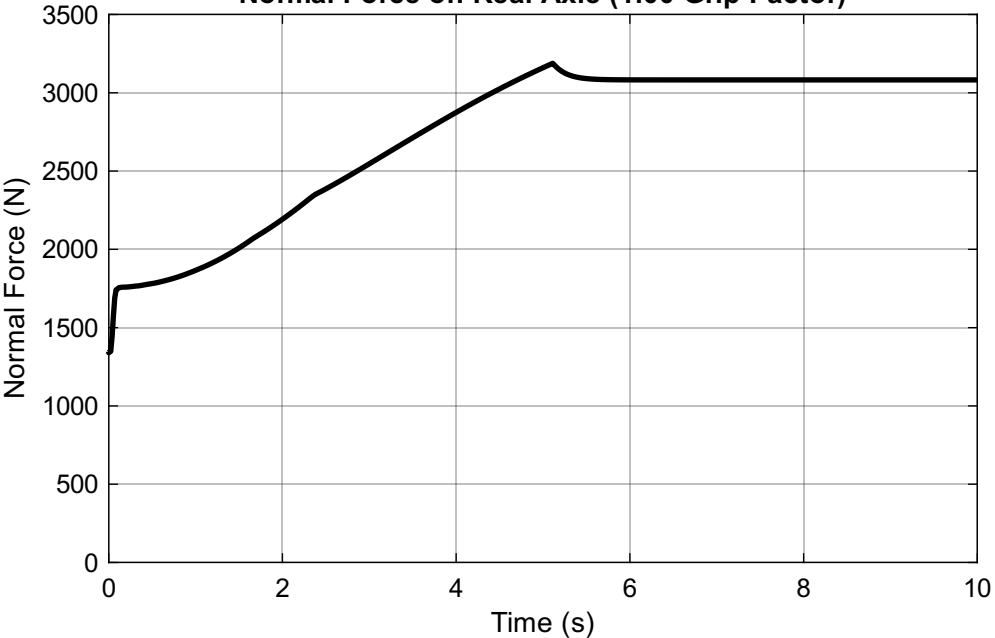
Normal Force on Rear Axle (1.00 Grip Factor)
