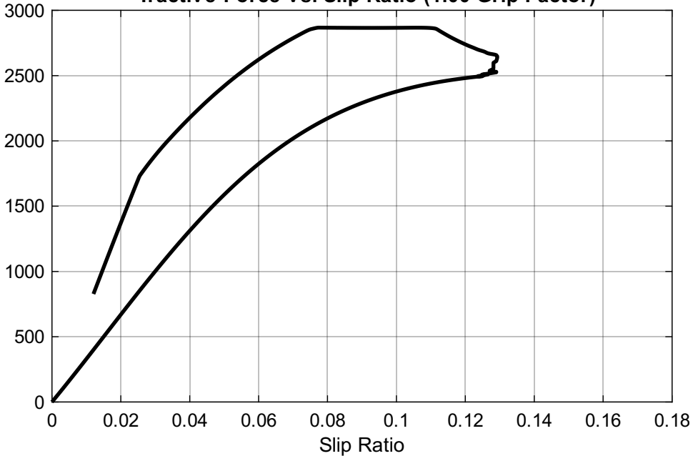
Tractive Force vs. Slip Ratio (1.00 Grip Factor)
