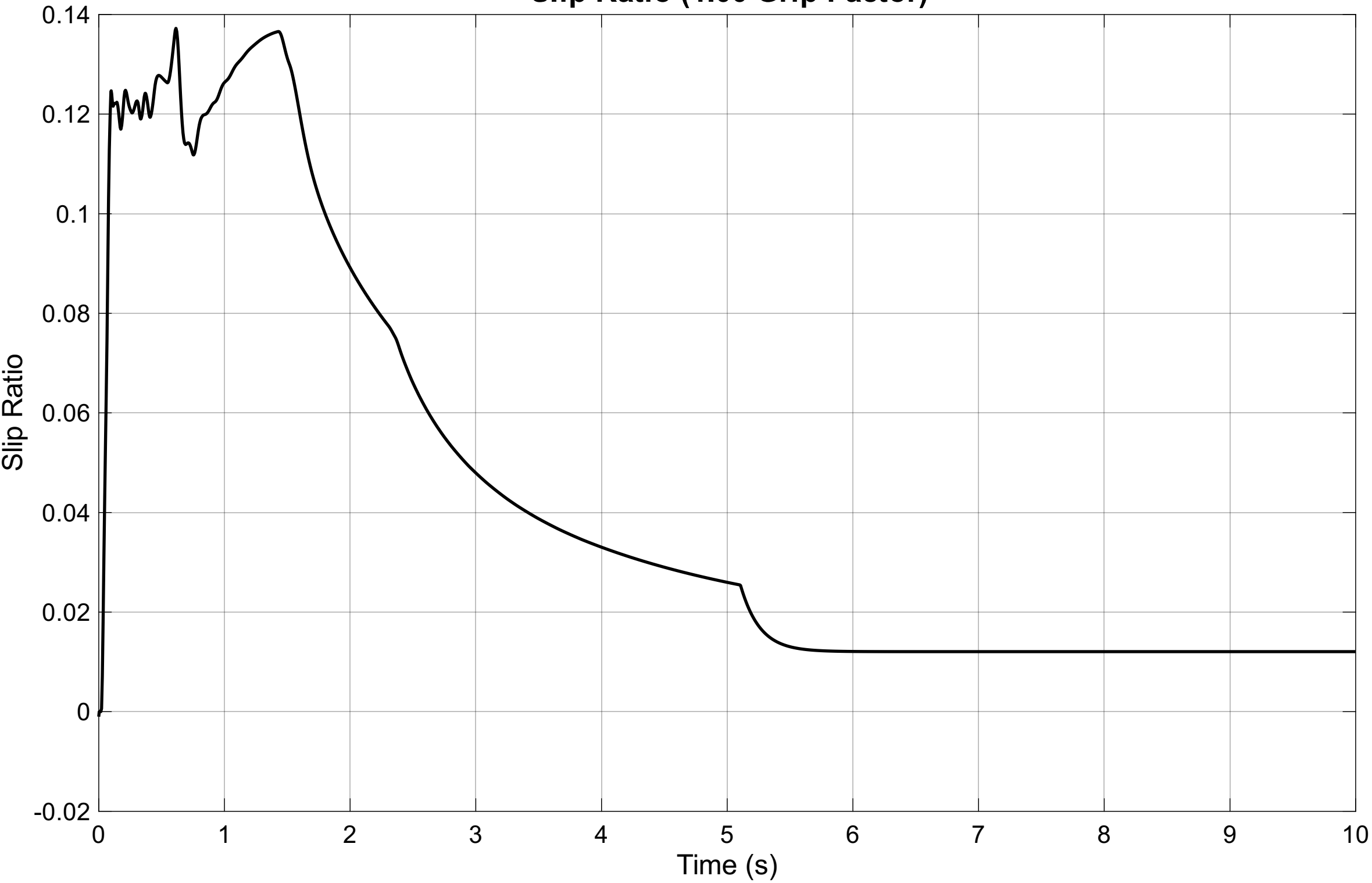
Slip Ratio (1.00 Grip Factor)
