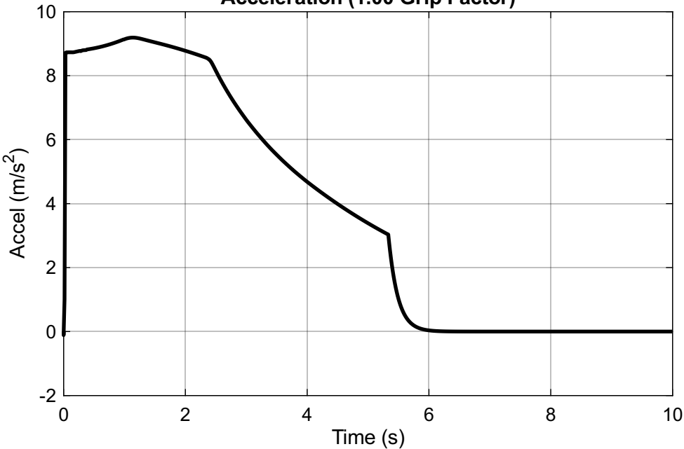
Acceleration (1.00 Grip Factor)
