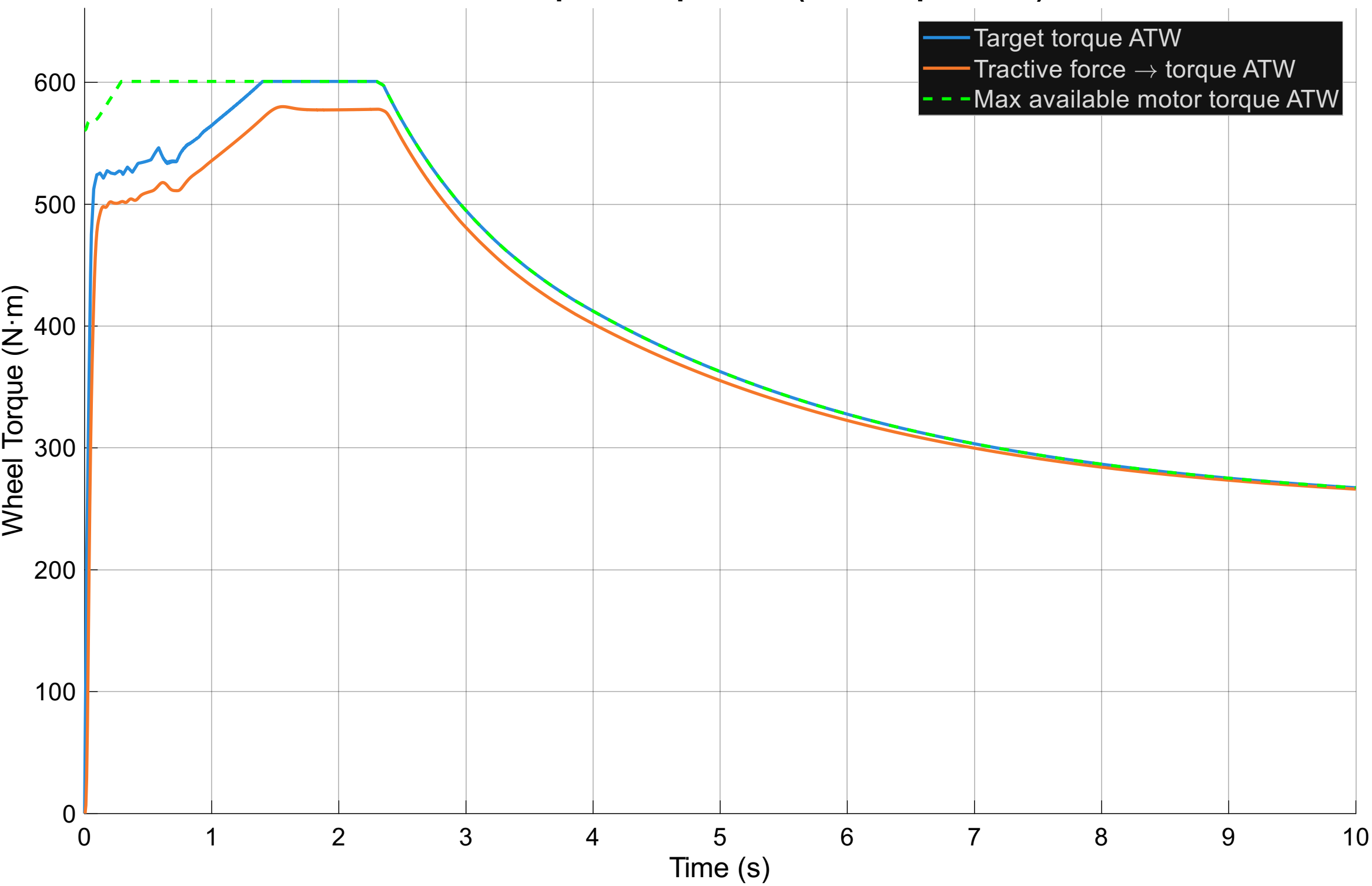
Wheel Torque Comparison (1.00 Grip Factor)
