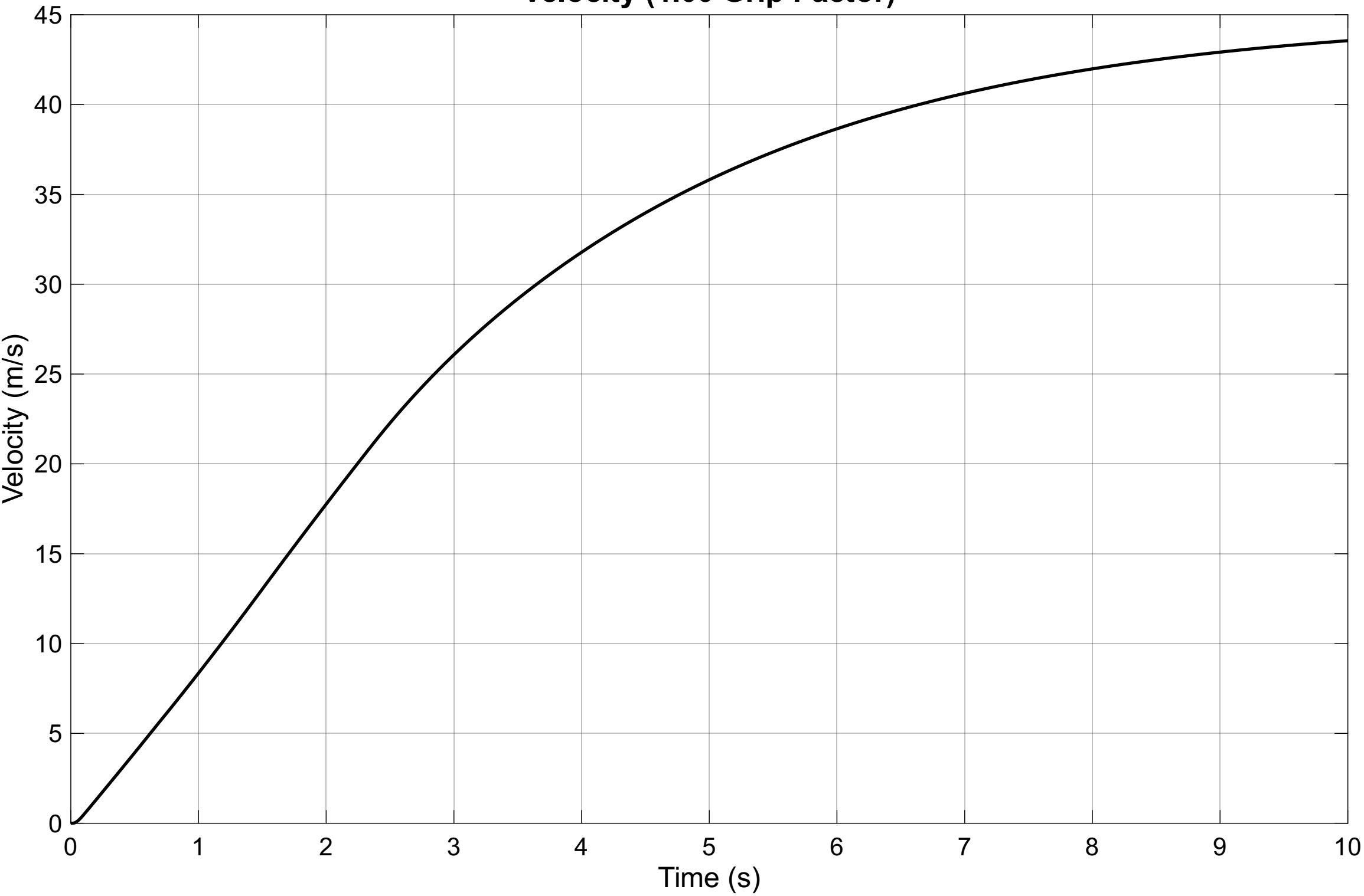
Velocity (1.00 Grip Factor)
