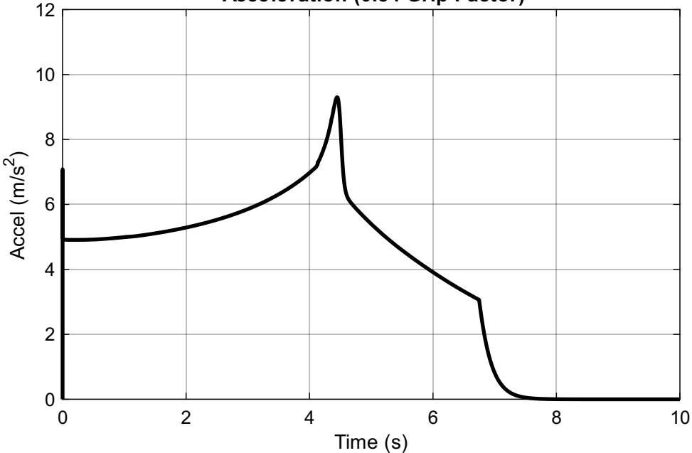
Acceleration (0.84 Grip Factor)
