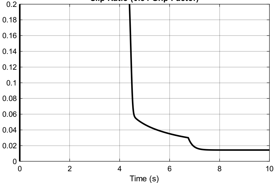
Slip Ratio (0.84 Grip Factor)
