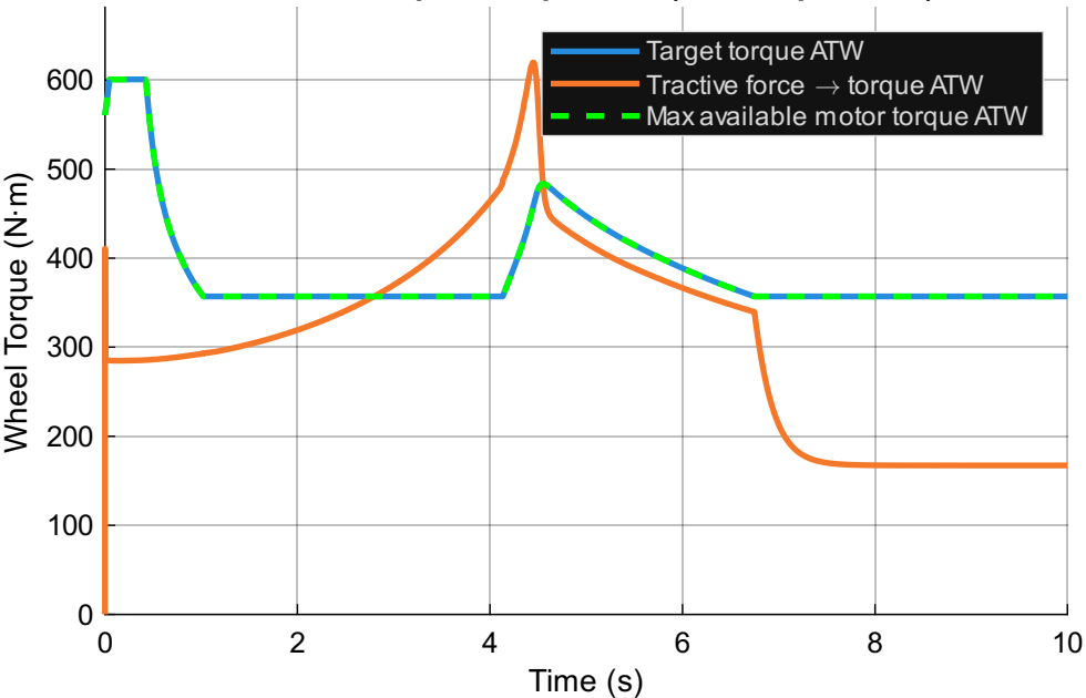
Wheel Torque Comparison (0.84 Grip Factor)
