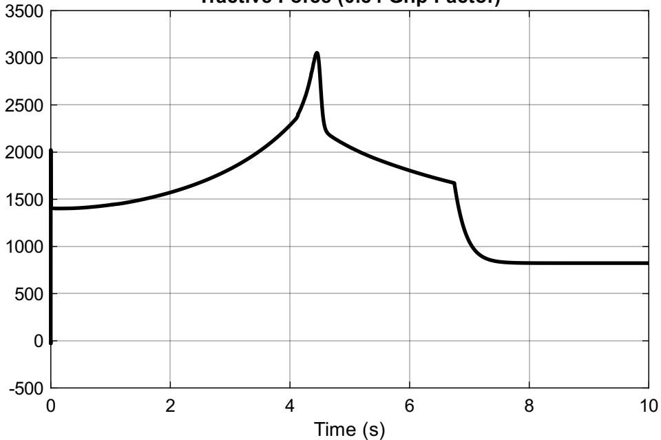
Tractive Force (0.84 Grip Factor)
