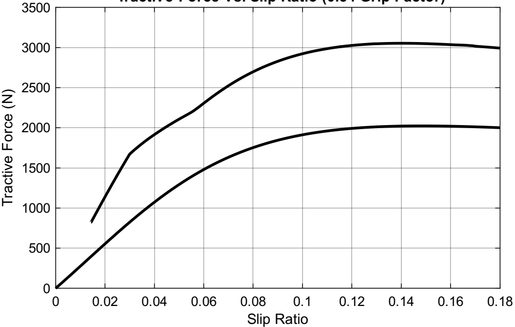
Tractive Force vs. Slip Ratio (0.84 Grip Factor)
