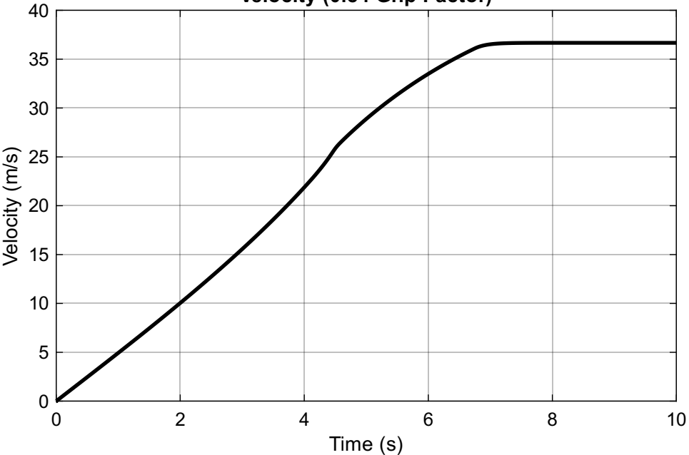
Velocity (0.84 Grip Factor)
