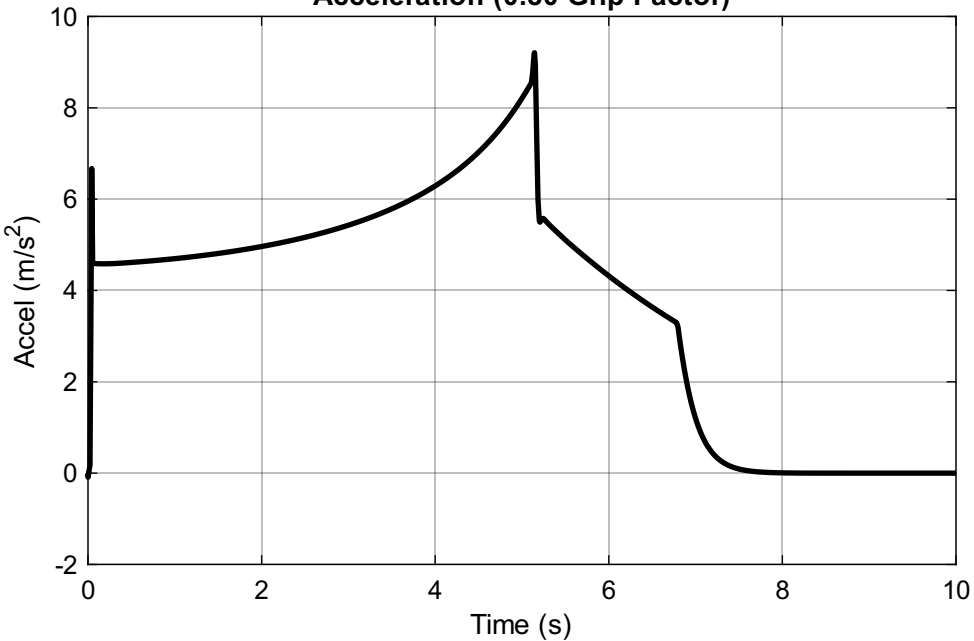
Acceleration (0.80 Grip Factor)
