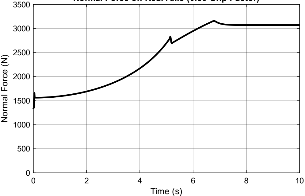
Normal Force on Rear Axle (0.80 Grip Factor)
