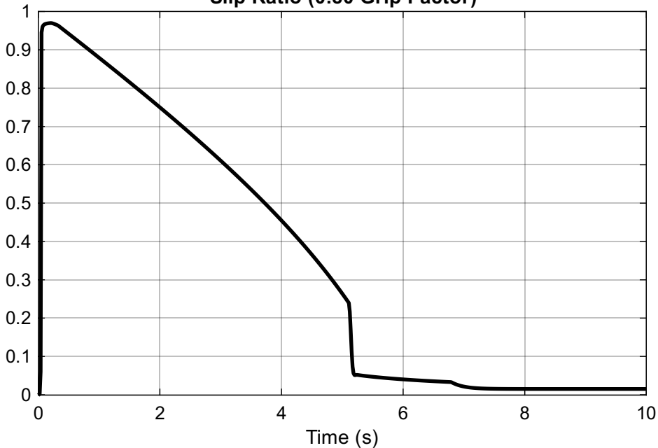
Slip Ratio (0.80 Grip Factor)
