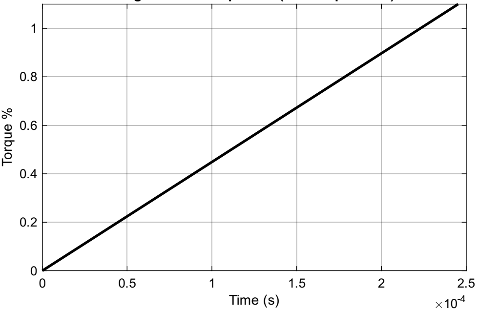
Target Motor Torque PID (0.80 Grip Factor)
