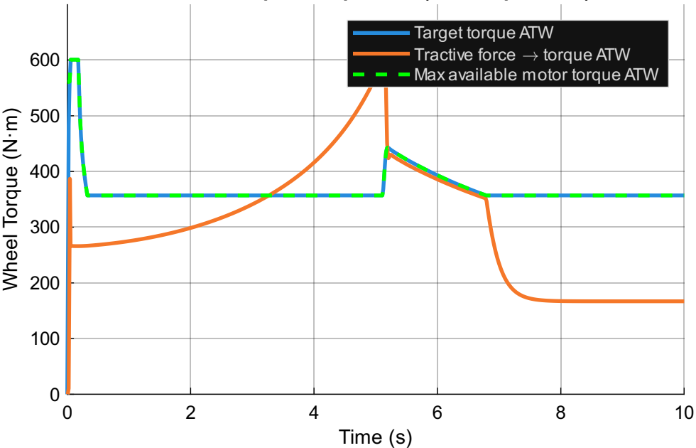
Wheel Torque Comparison (0.80 Grip Factor)
