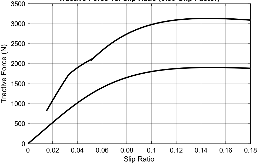
Tractive Force vs. Slip Ratio (0.80 Grip Factor)
