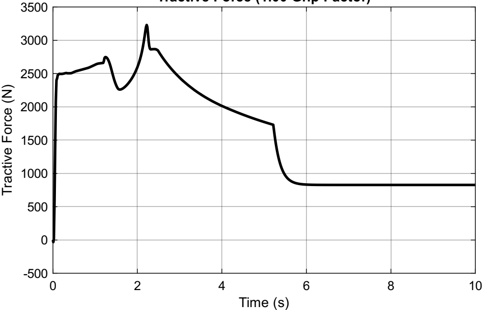
Tractive Force (1.00 Grip Factor)
