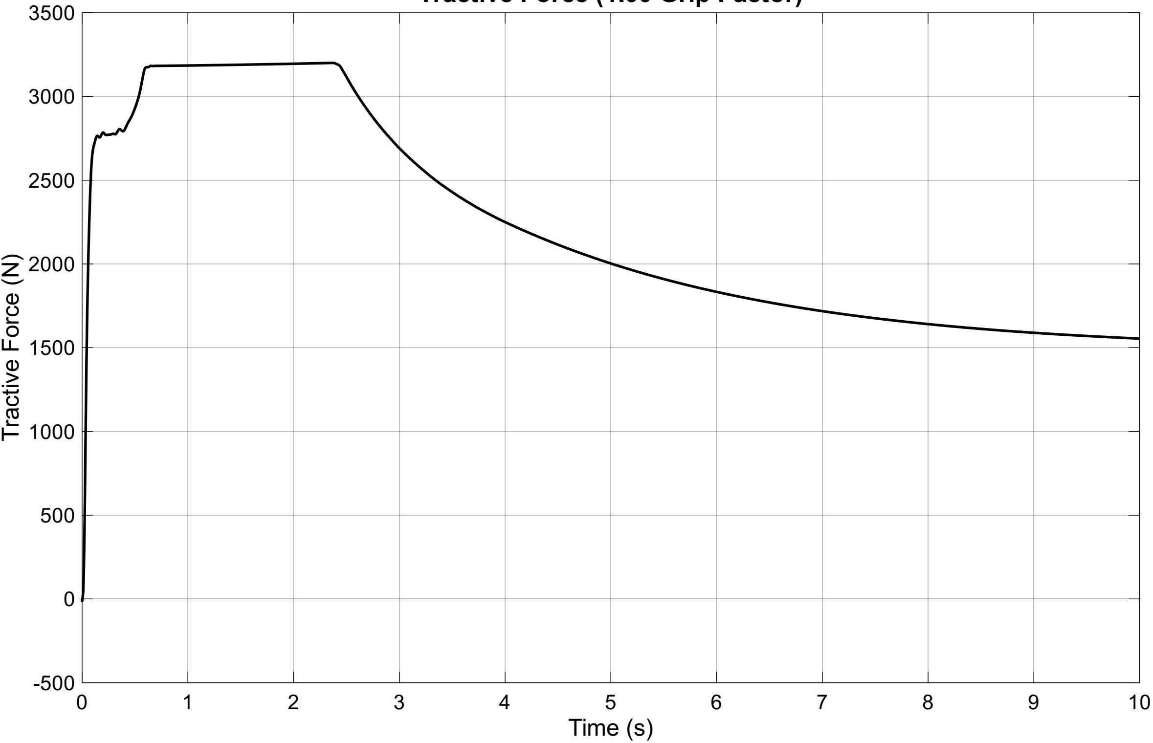
Tractive Force (1.00 Grip Factor)
