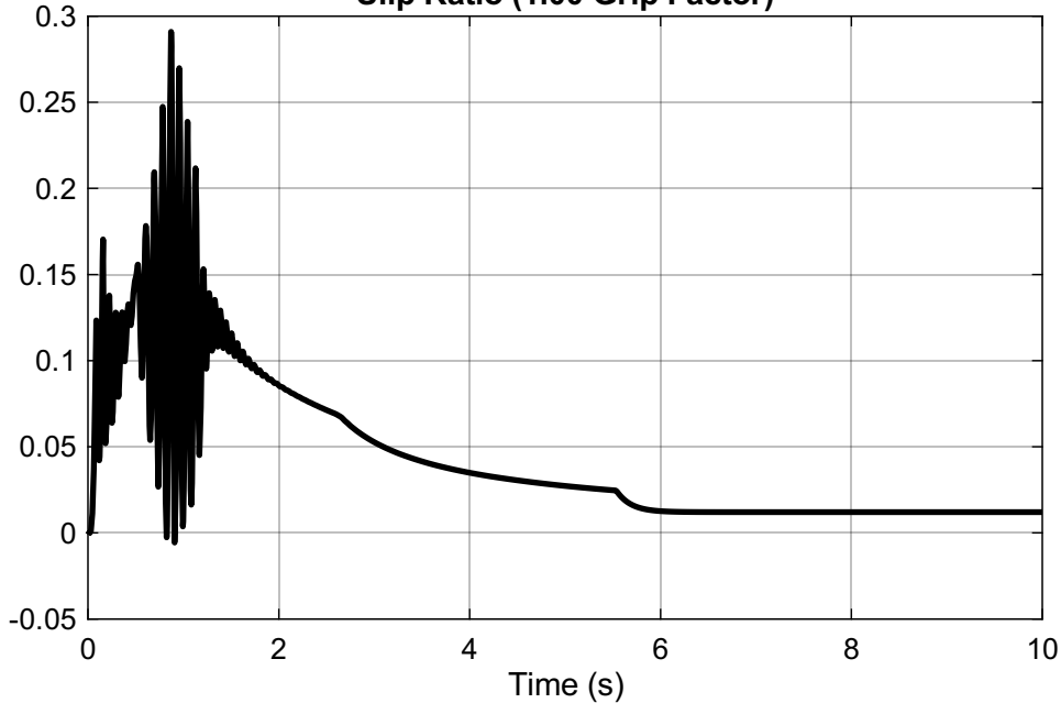
Slip Ratio (1.00 Grip Factor)
