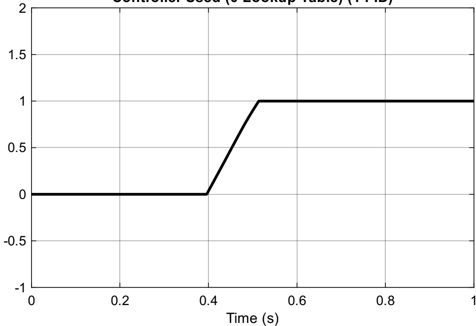
Controller Used (0 Lookup Table) (1 PID)
