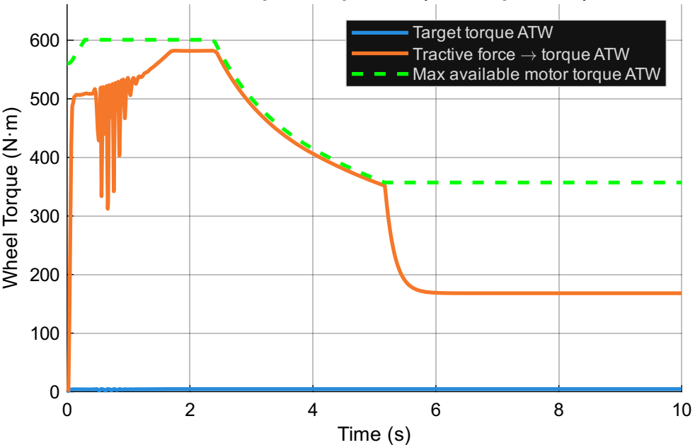
Wheel Torque Comparison (1.00 Grip Factor)
