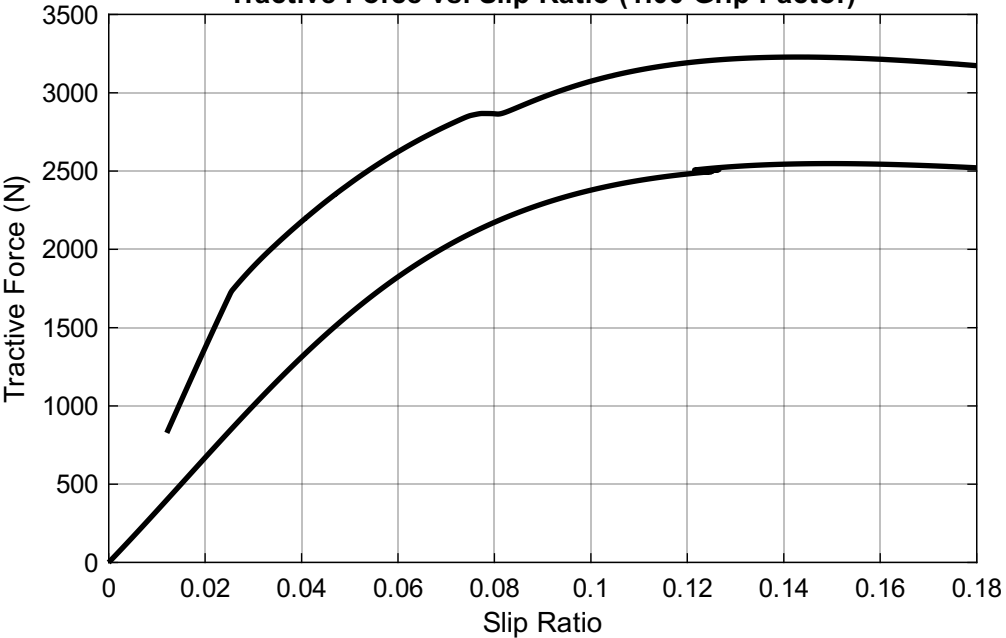
Tractive Force vs. Slip Ratio (1.00 Grip Factor)
