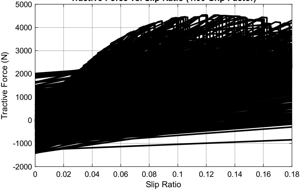
Tractive Force vs. Slip Ratio (1.00 Grip Factor)
