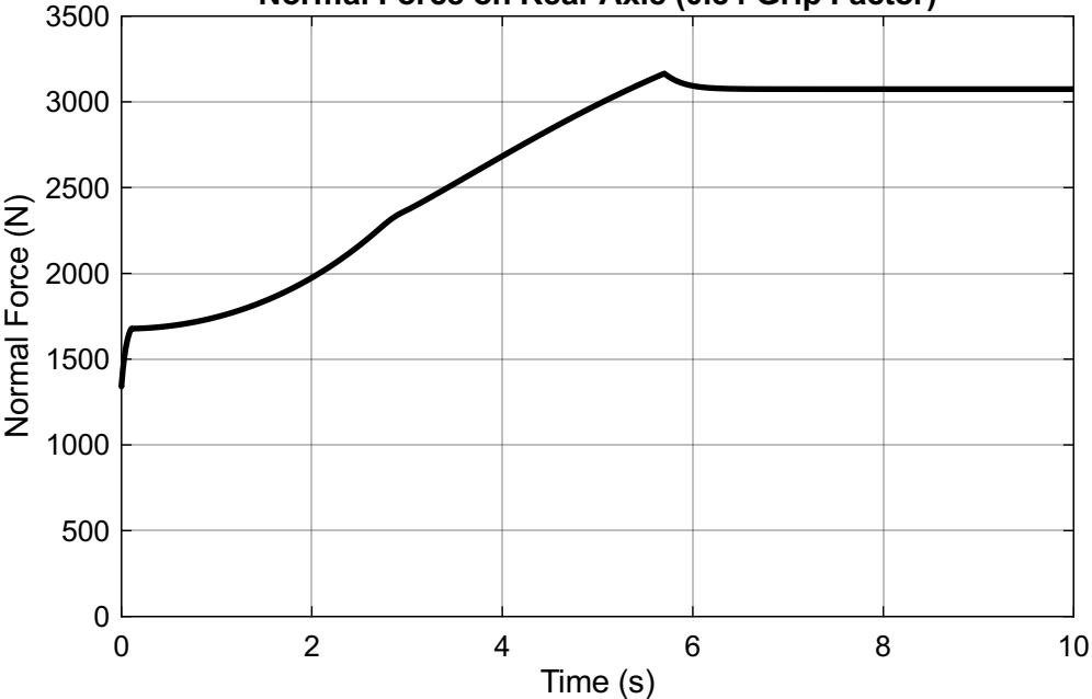
Normal Force on Rear Axle (0.84 Grip Factor)
