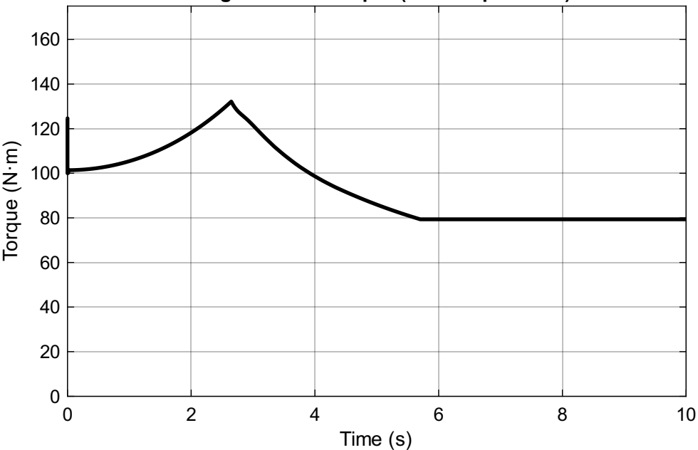
Target Motor Torque (0.84 Grip Factor)
