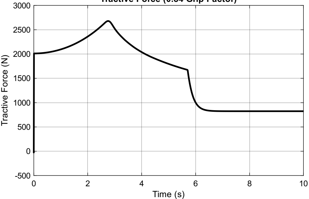
Tractive Force (0.84 Grip Factor)
