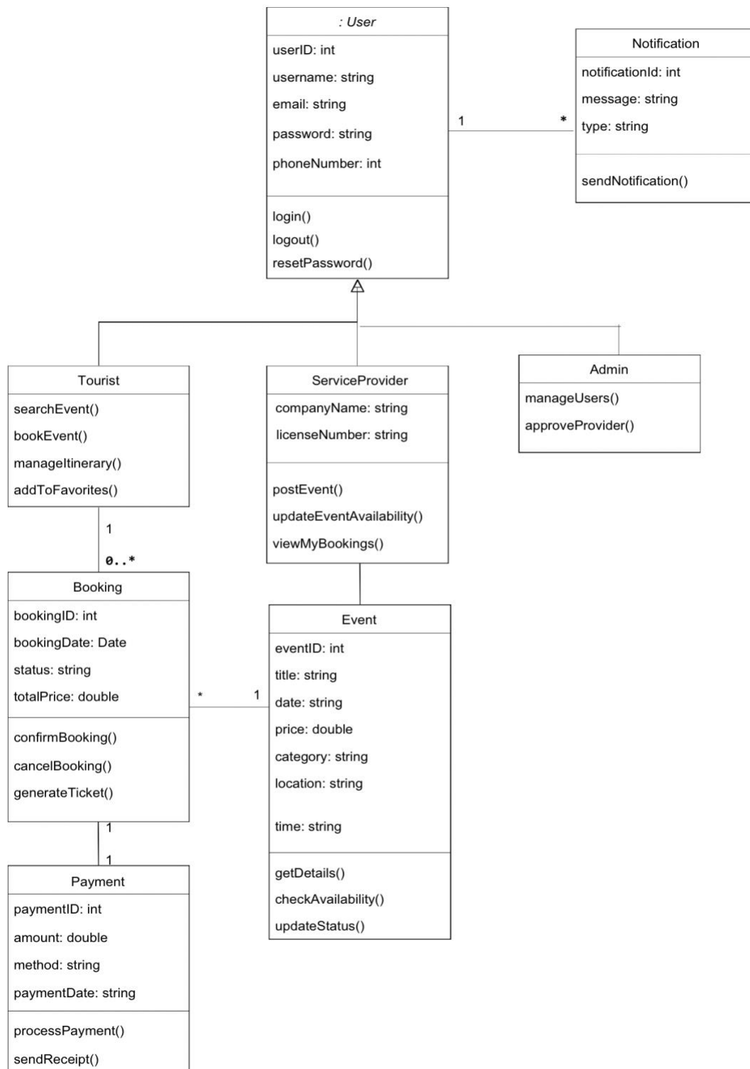
Figure 3: Class Diagram
