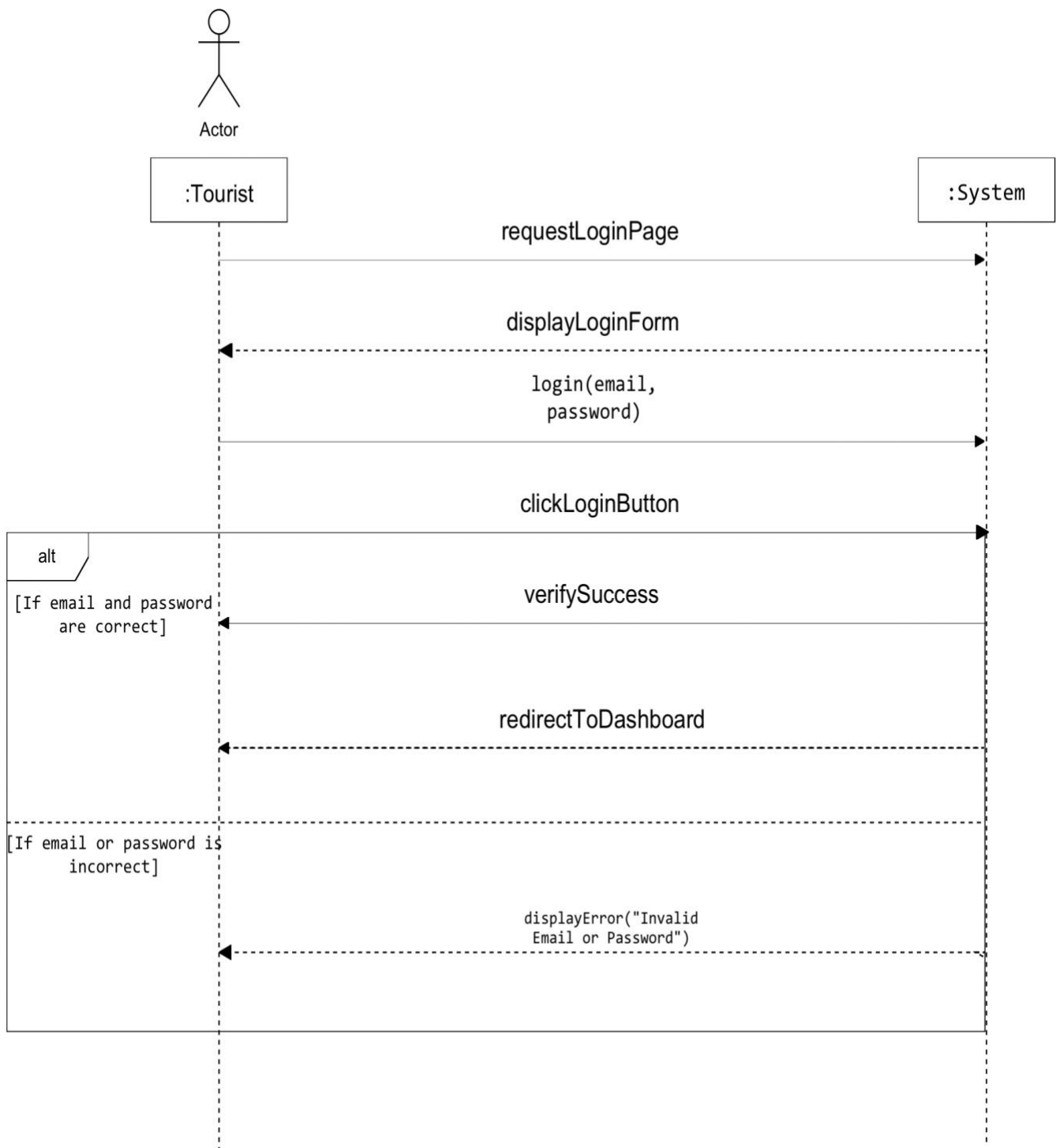
Figure 2: System Sequence Diagram
