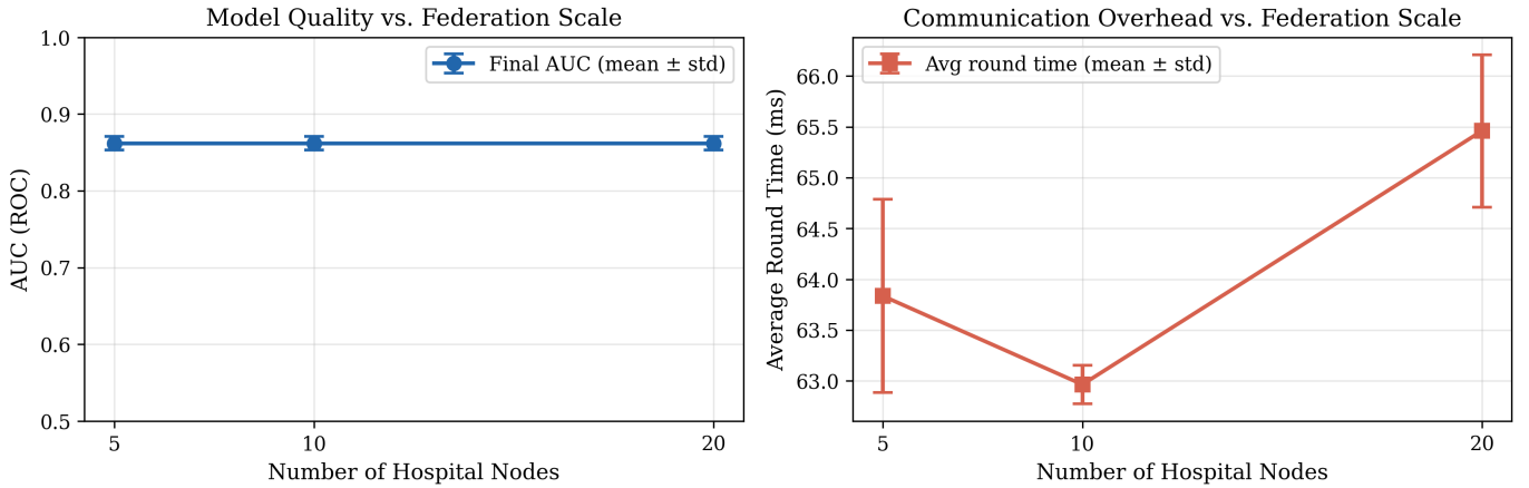
Fig. 6. Scalability of PQC-FL-Health (50 rounds, 3 seeds, ML-KEM-768 + ML-DSA-65). Left: Final AUC vs. federation size. AUC remains stable at 0.862 \pm 0.010 across 5, 10, and 20 nodes; error bars show std across seeds. Right: Average per-round latency. Latency is flat at 63–65 ms regardless of node count, confirming that PQC overhead does not compound with federation size.
