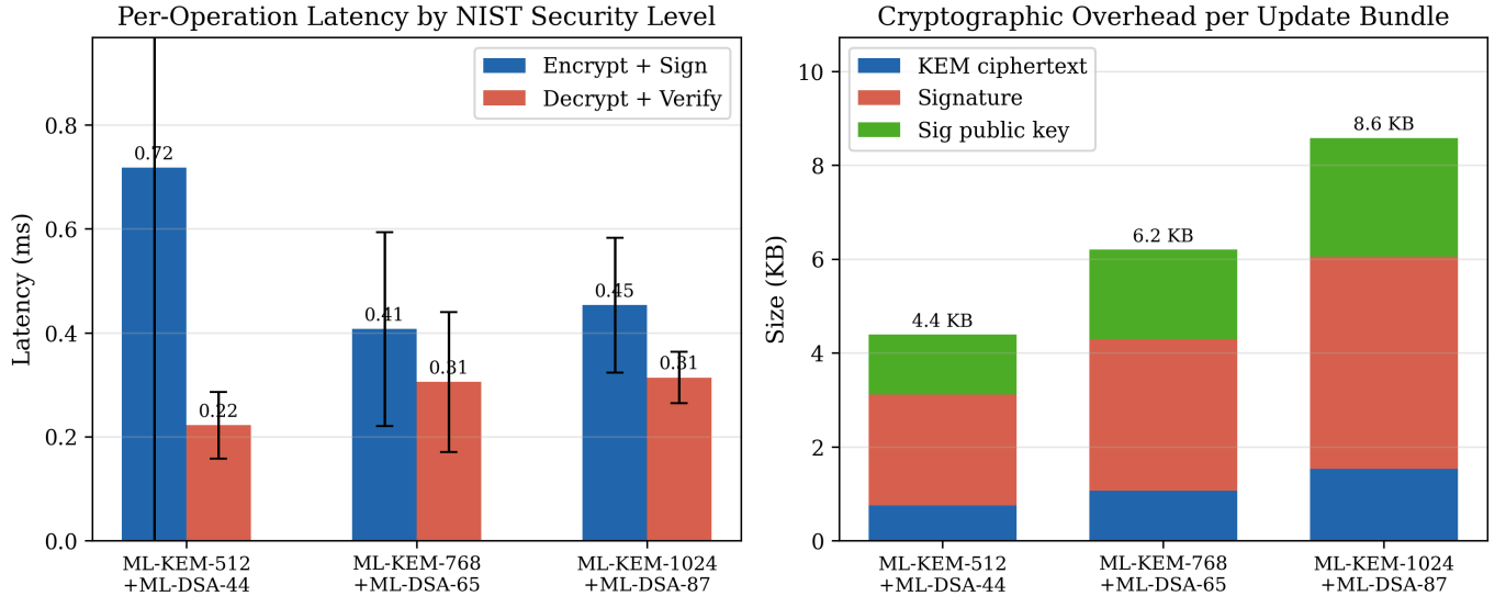
Fig. 3. NIST post-quantum security level comparison on a 12 KB model-delta payload (20 iterations each). Left: Per-operation latency (mean \pm std). All levels complete encrypt+sign and decrypt+verify under 0.8 ms. Right: Cryptographic overhead per update bundle, broken down into KEM ciphertext, signature, and signing public key. Overhead ranges from 4.4 KB (Level 1) to 8.6 KB (Level 5).
