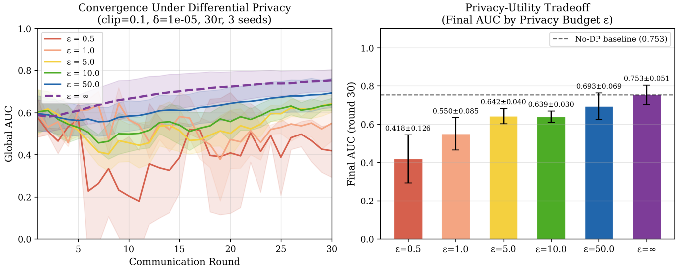
Fig. 5. Differential privacy tradeoff (30 rounds, 3 seeds, clip S = 0.1 , \delta = 10^{-5} ). Shaded bands show \pm 1 std across seeds. Left: Mean convergence curves per \epsilon . Right: Final AUC (mean \pm std) vs. privacy budget. At \epsilon \geq 5 , AUC is 0.64–0.75. At \epsilon \leq 1 , noise causes both degradation and high variance, making convergence unpredictable.
