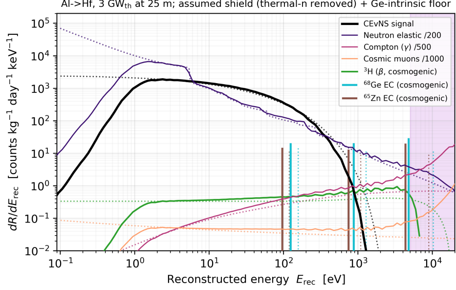
FIG. 1. Central result: reconstructed-energy differential rate spectra dR/dE_{\text{rec}} (counts \text{kg}^{-1} \text{day}^{-1} \text{keV}^{-1} ) for the Al→Hf design under non-paralyzable censoring, in the assumed-shield scenario (Ta→Al is qualitatively identical). The reconstructed energy is calibrated to estimate the deposited energy. The reactor-CEvNS signal (black, thick) reconstructs to tens of eV. The ambient neutron-elastic recoils (purple) occupy the same band and, even after the assumed neutron suppression factor of 200 shown, are the dominant background there; cosmic-muon deposits (orange, suppressed by the assumed factor 1000 veto) span \sim 1.5 –197 MeV yet pile up at tens of keV—an instrumental artifact of the bandwidth ceiling, not a physical line; the environmental-gamma Compton continuum (magenta, suppressed by the assumed factor 500) fills the region between. The Ge-intrinsic cosmogenic floor— ^3\text{H} (green), ^{68}\text{Ge} and ^{65}\text{Zn} electron-capture lines (cyan and brown stems)—is drawn unsuppressed, as no external shield reaches it. Solid curves are the reconstructed (saturated, triggered) spectra; dotted curves are the corresponding linear-response, pre-saturation forms. Shaded purple marks the bandwidth-saturated region. The suppression factors are the assumed-shield modeling inputs of Sec. IV, quoted in the legend.
