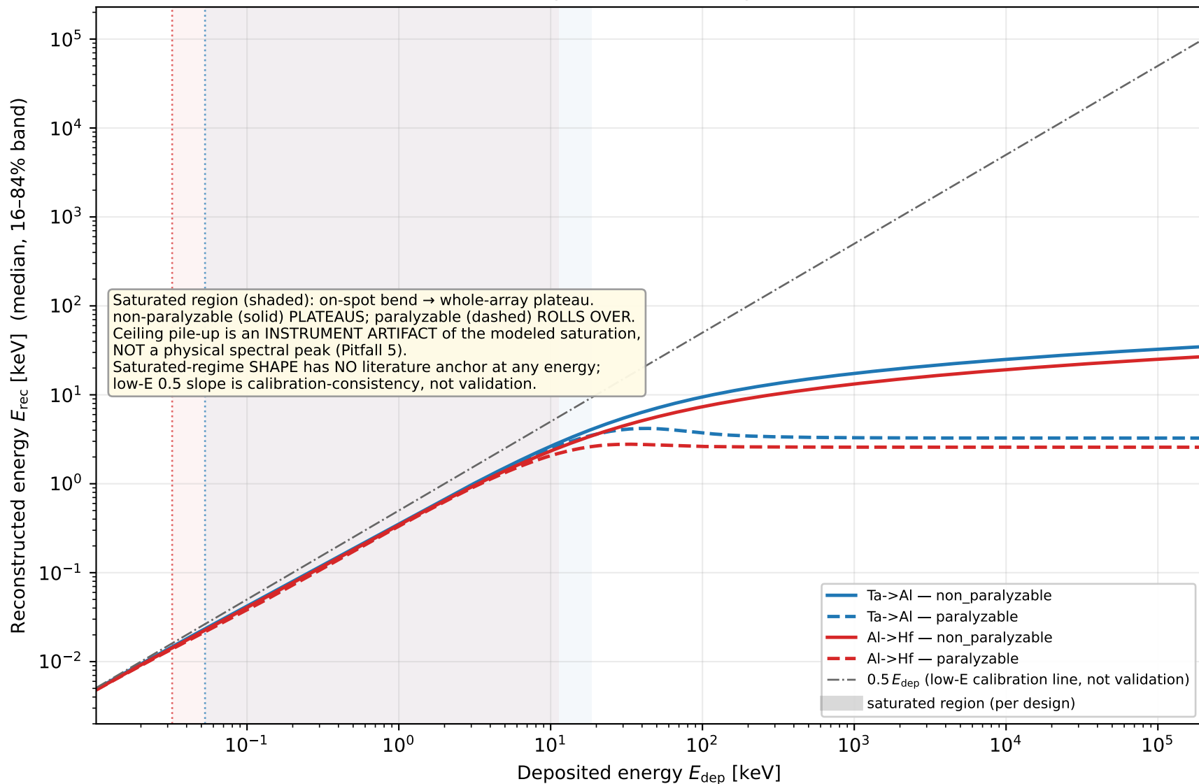
QPD bandwidth-limited response R(E_{\text{rec}} | E_{\text{dep}}) : linear \rightarrow saturated (both designs, both censoring variants)
