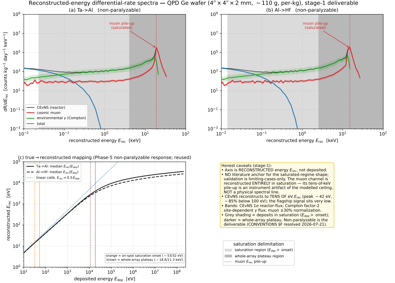
FIG. 1. Reconstructed-energy differential rate spectra dR/dE_{\text{rec}} (counts \text{kg}^{-1} \text{day}^{-1} \text{keV}^{-1} ) for the two QPD trapping designs, (a) Ta→Al and (b) Al→Hf, under non-paralyzable censoring. Reactor CEvNS (blue) reconstructs to tens of eV; cosmic muons (red) pile up at the saturation plateau (tens of keV, an instrumental artifact of the bandwidth ceiling); environmental-gamma Compton (green) fills the continuum between; the total is shown in black. Shaded bands are the propagated flux uncertainties; grey shading marks the saturation region. Panel (c) shows the true-to-reconstructed energy mapping. Nothing below 10 eV is displayed.
