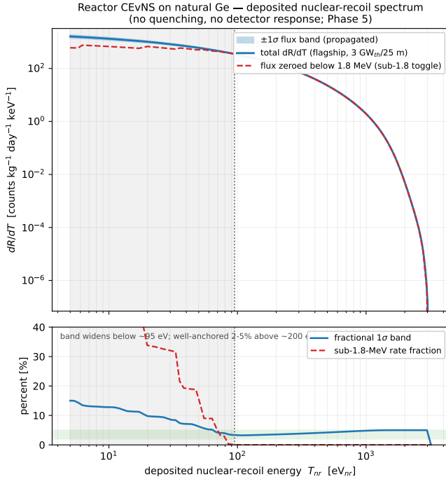
FIG. 3. Deposited nuclear-recoil differential CEvNS rate dR/dT on natural germanium at 3 \text{GW}_{\text{th}} and 25 m, with the split flux-uncertainty band and the Billard-benchmark reproduction.
