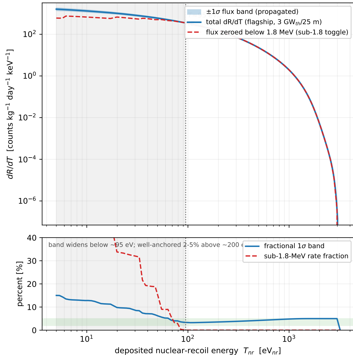
Reactor CEvNS on natural Ge — deposited nuclear-recoil spectrum (no quenching, no detector response; Phase 5)
