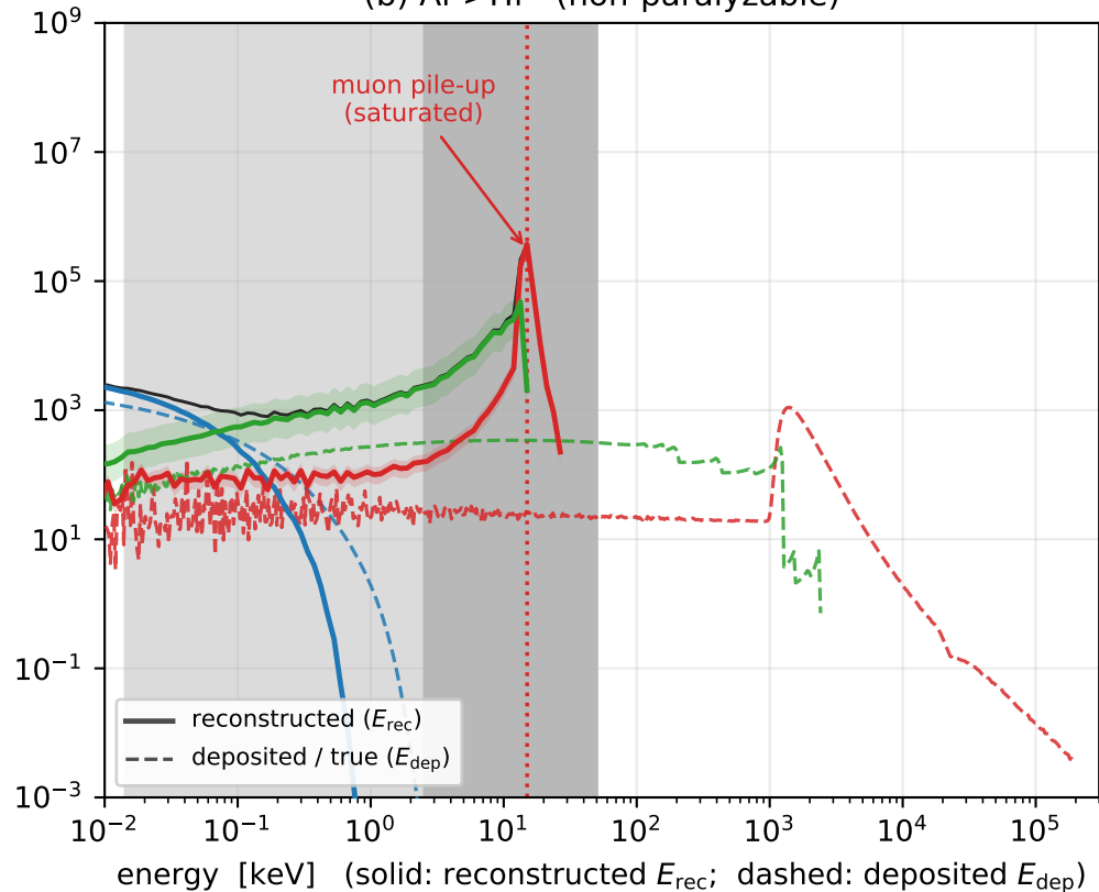
(b) Al-&gt;Hf (non-paralyzable)
