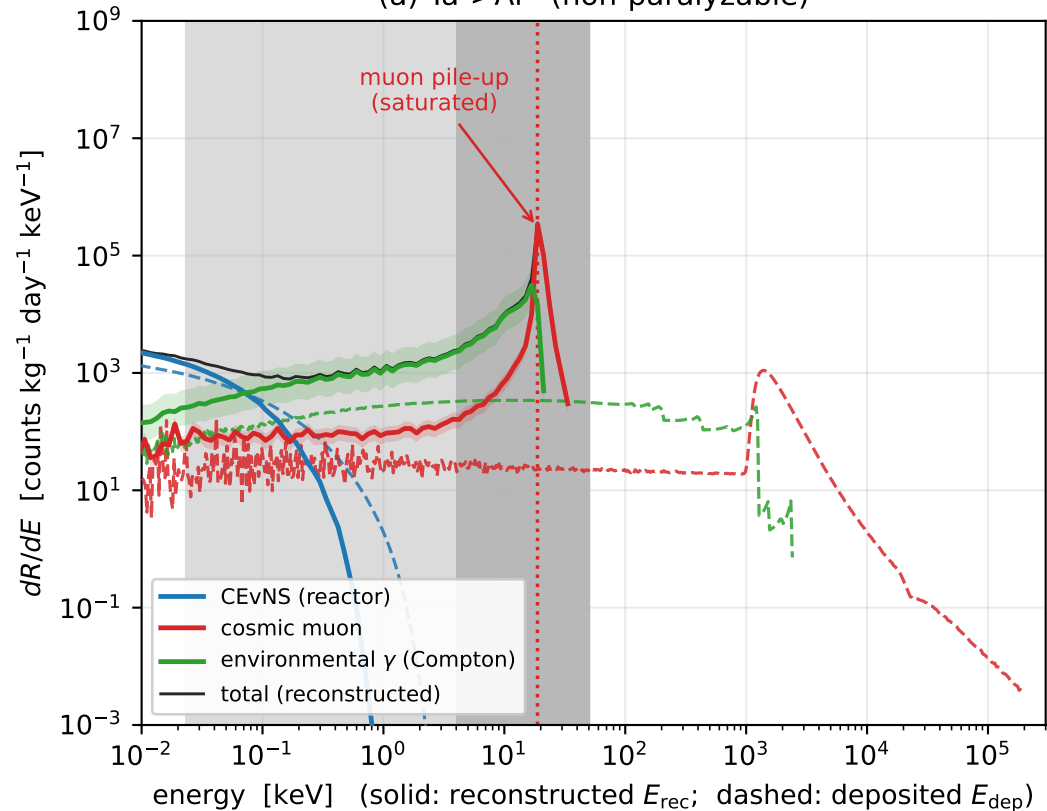
(a) Ta-&gt;Al (non-paralyzable)
