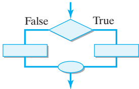
Selection if/else
