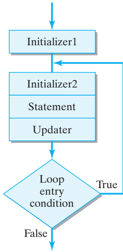
Do-While Structure
