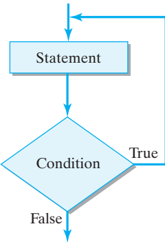
Do-While Statement
