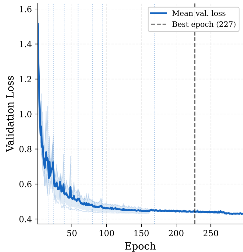
LSTM
