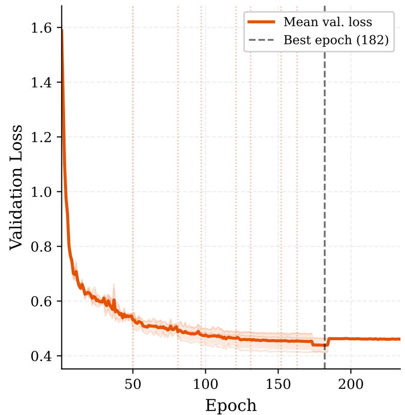
Transformer
